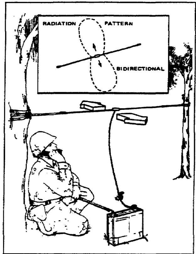
Figure 2-3. Half-wave doublet antenna supported by trees
