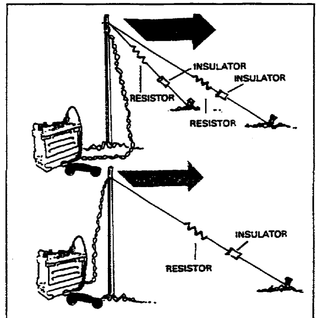
Figure 2-30. Sloping-V antenna
