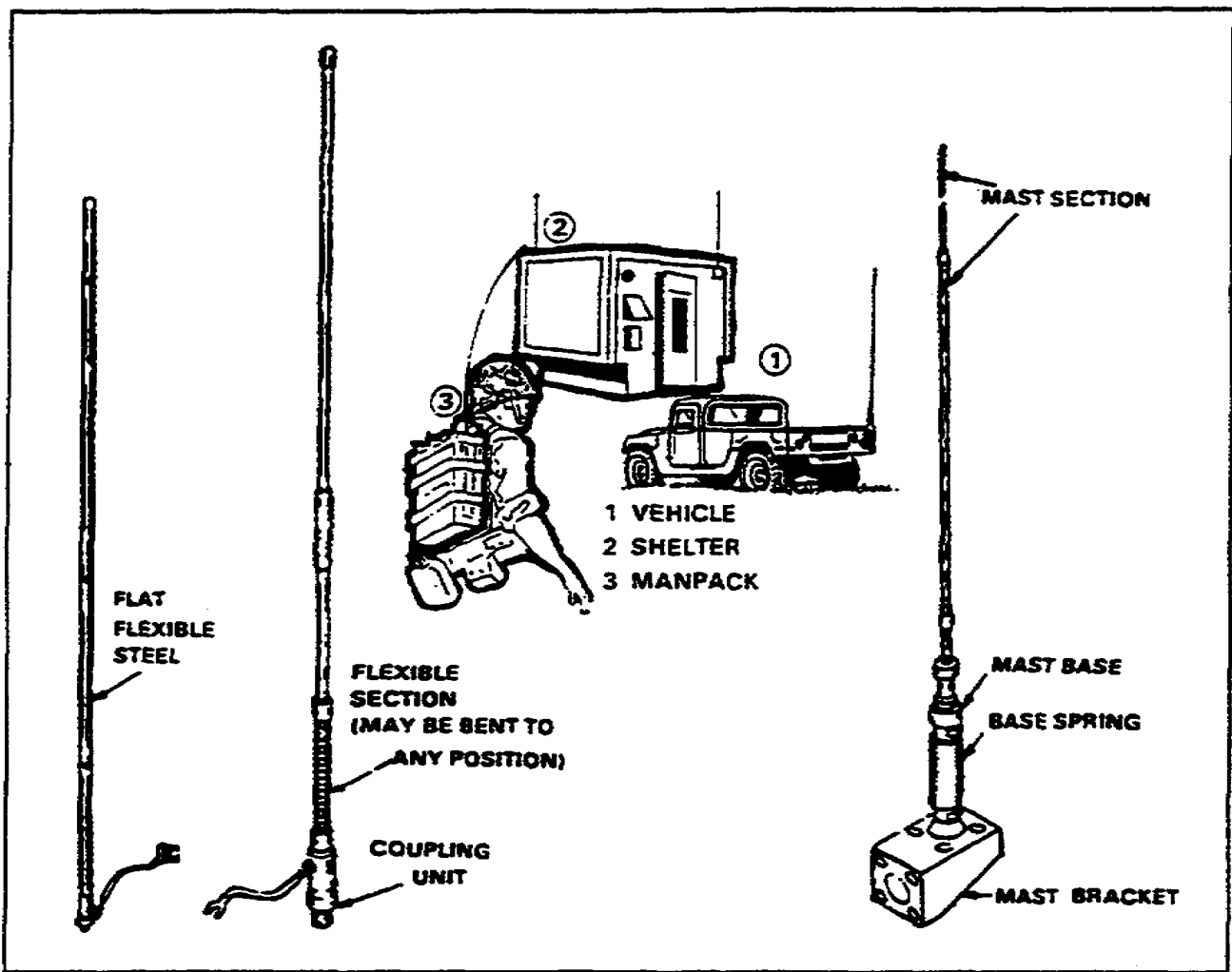
Figure 2-4. Whip antennas
