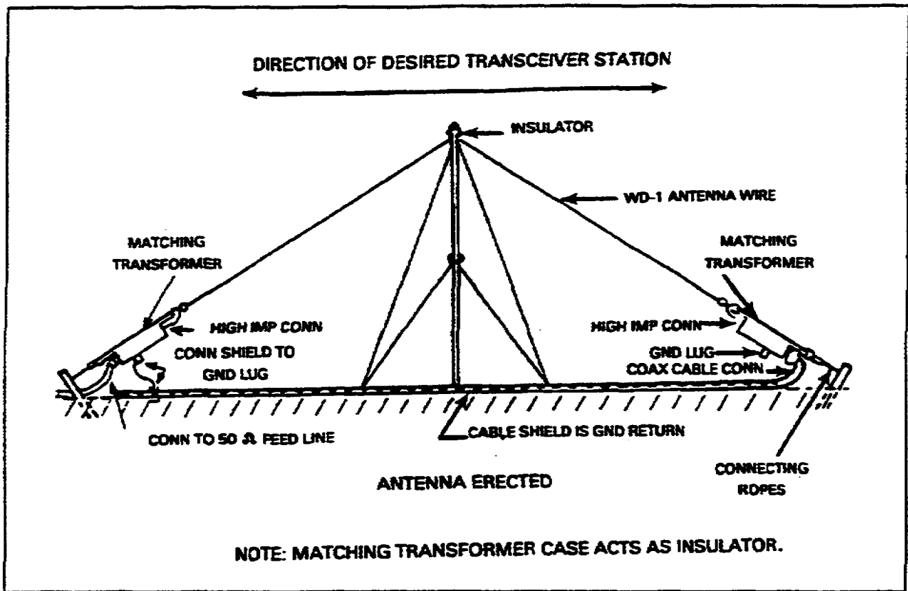
Figure 2-9. Half-rhombic VHF antenna
