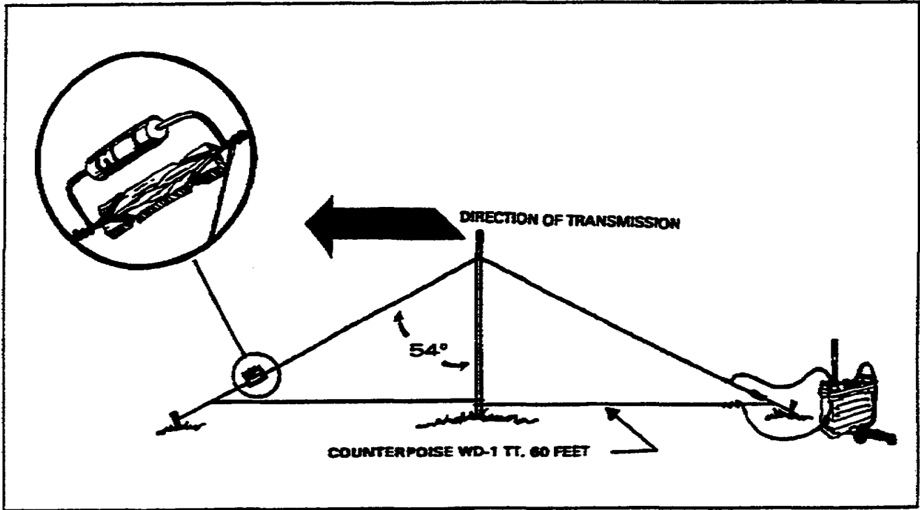
Figure 2-27. Vertical half-rhombic antenna
