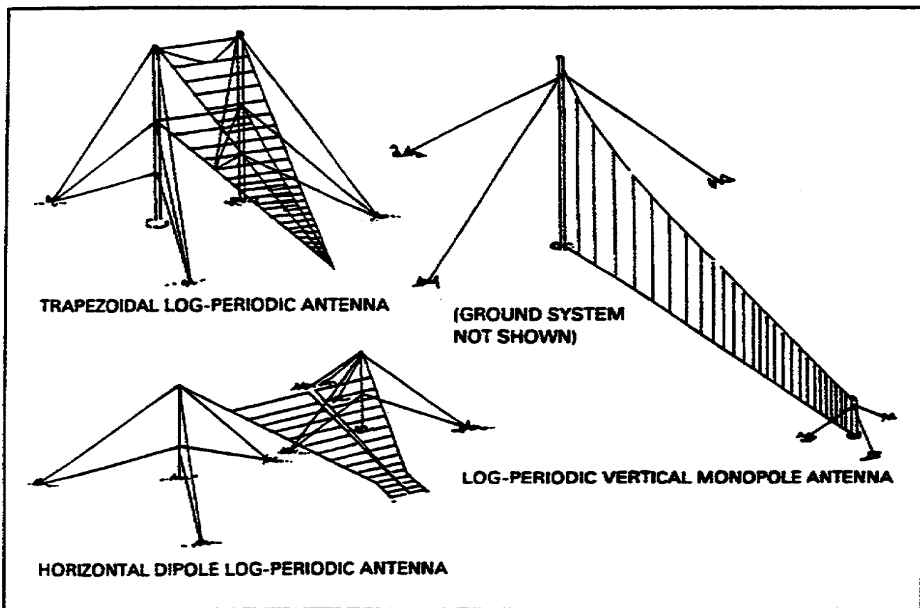
Figure 2-8. Log-periodic antenna
