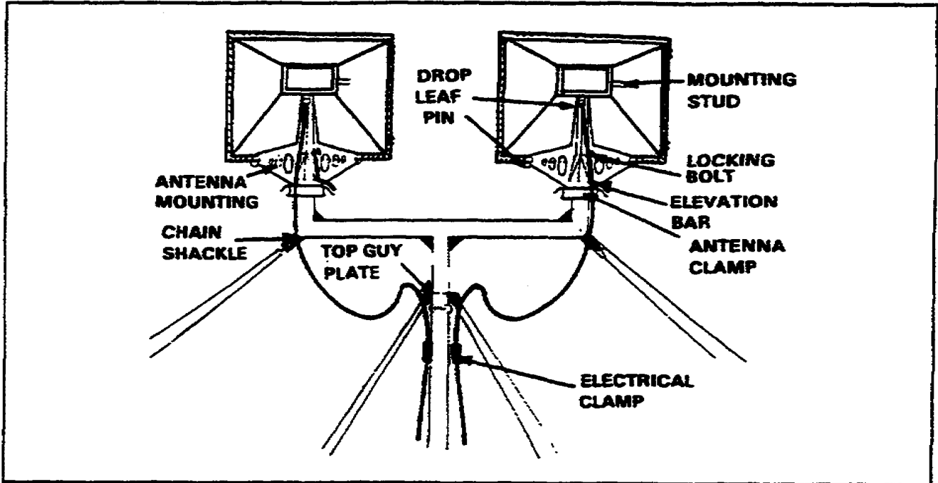
Figure 2-18. Typical horn-type antenna
