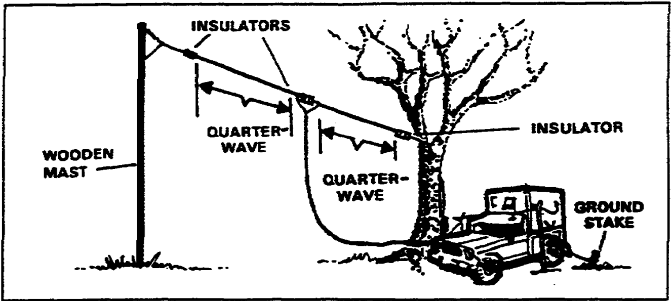
Figure 2-25. Half-wave doublet antenna
