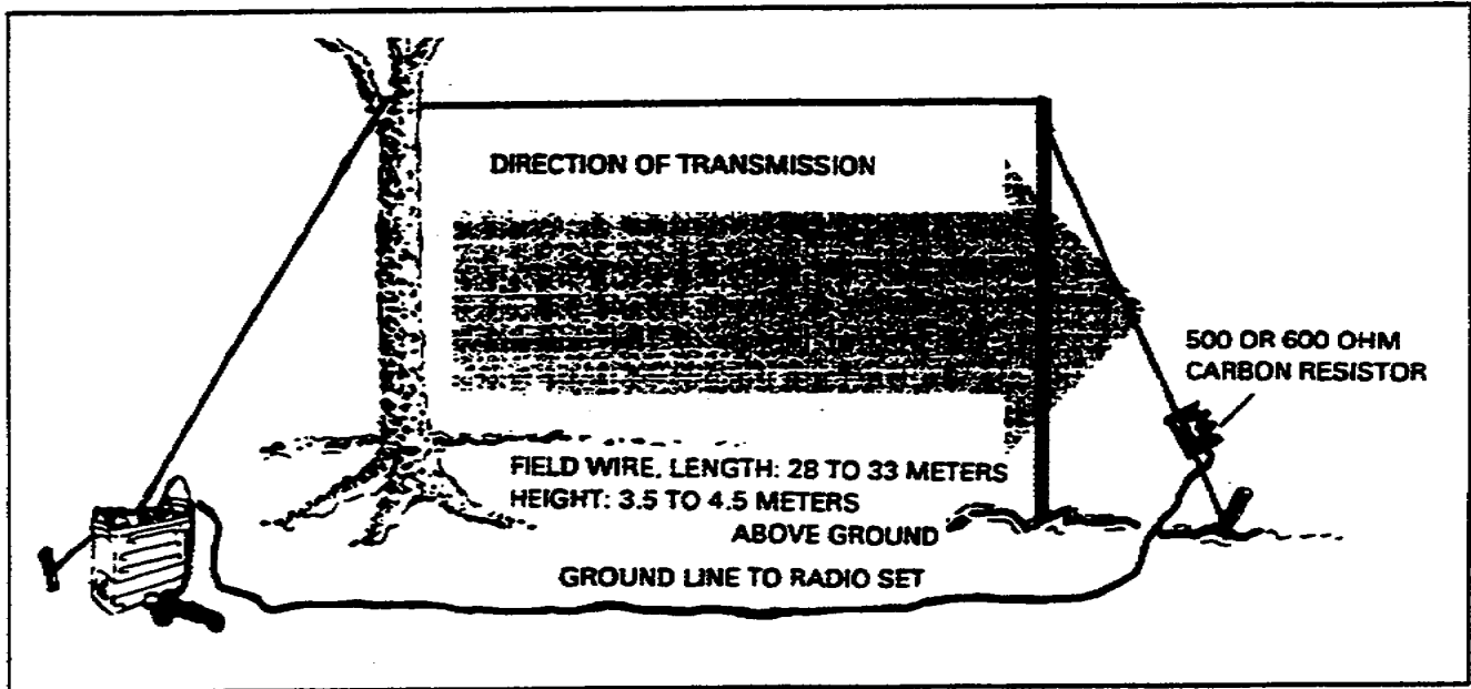
Figure 2-28. Long-wire antenna
