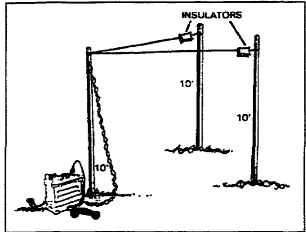
Figure 2-29. V antenna
